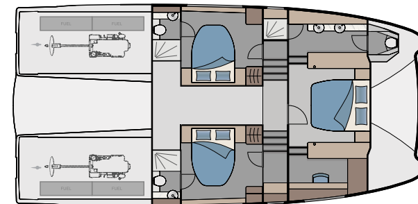
STANDARD 2 CABIN / 3 HEAD
