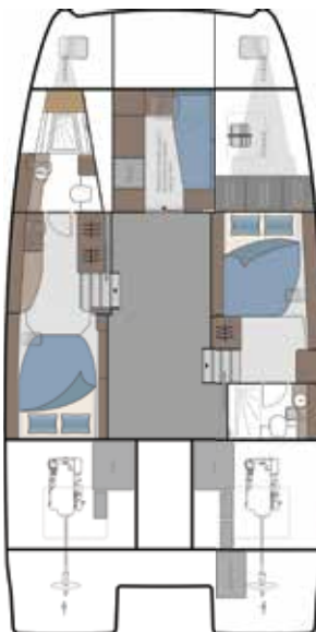
STANDARD 2 CABIN + UTILITY
